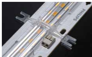
C14353_FLORENCE-1R-CLIP-A for 40.1 mm wide PCB's and screw mount
